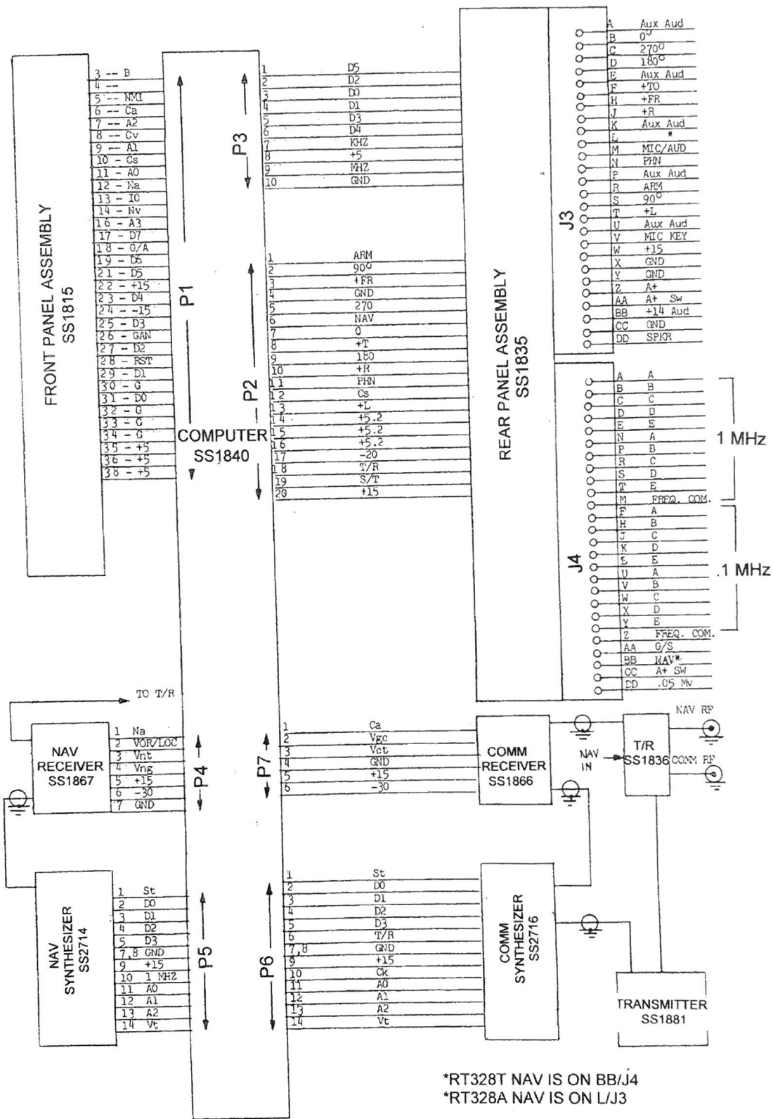
FIGURE 5 MX300 INTERCONNECT
